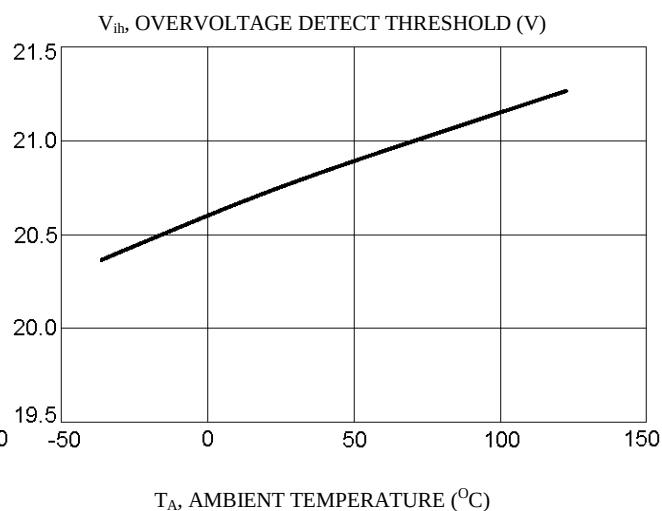
Figure 4 – Overvoltage Detector versus Temperature
