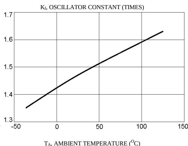
Figure 8 – Oscillator Constant versus Temperature
